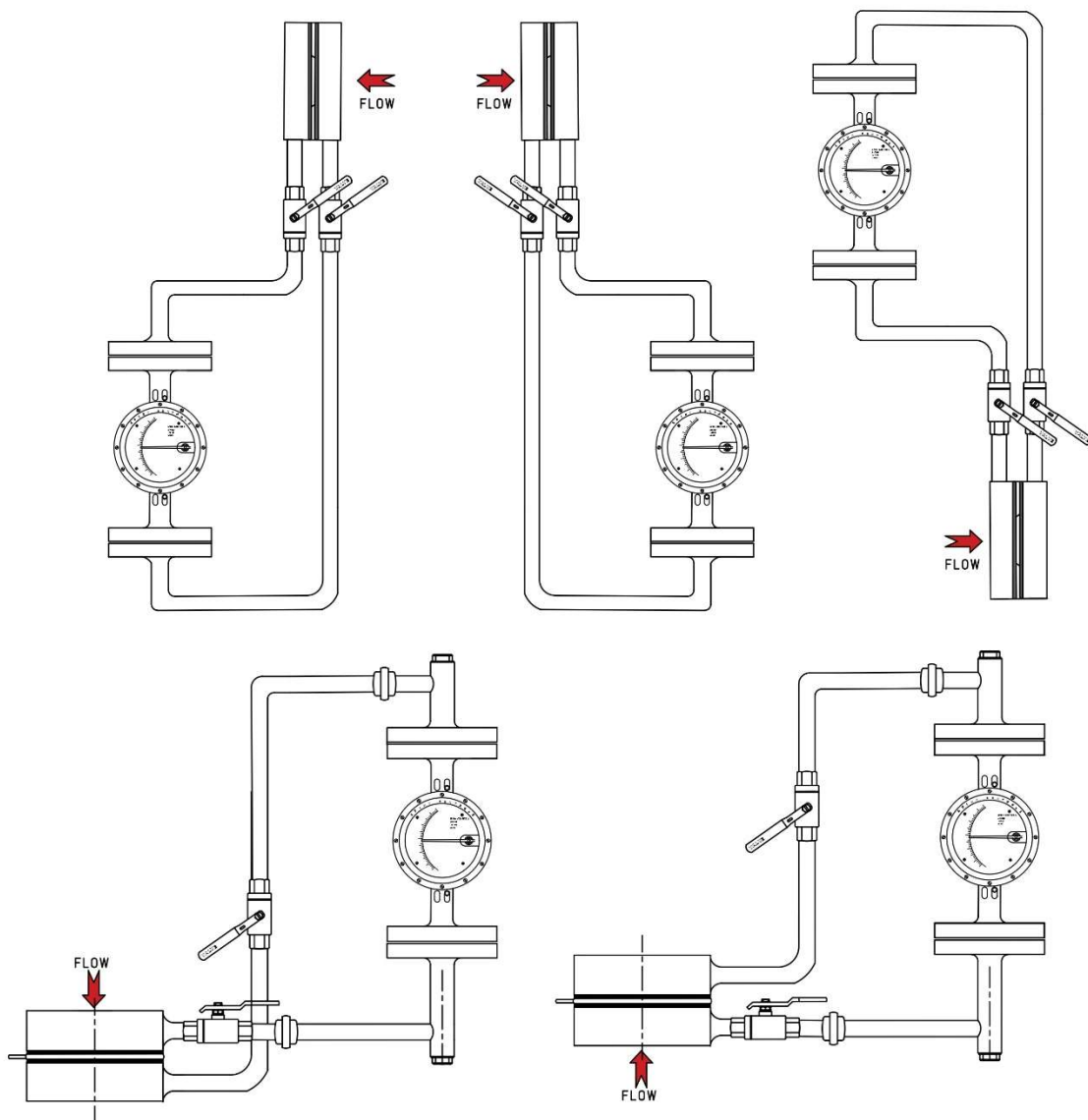
Fig No.: 4.2 – By pass type Flowmeter types
