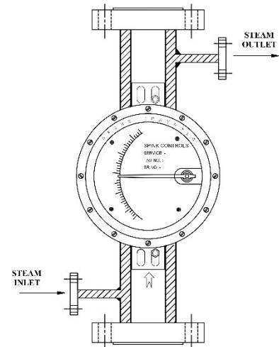
Fig No.: 4.2 – Steam jacketing type Flowmeter
